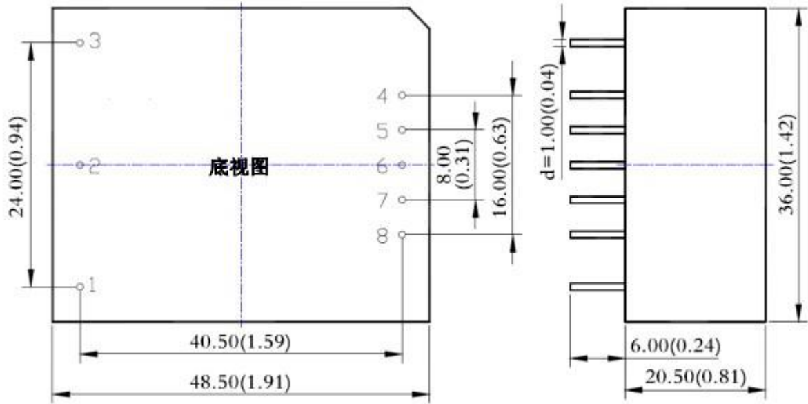
BOTTOM VIEW
