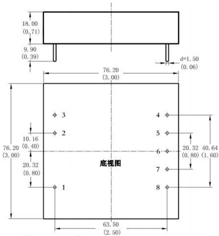
BOTTOM VIEW
